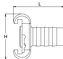
Coupling with hose connection
