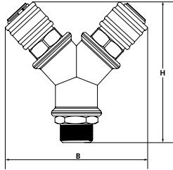
Distributor with 2 quick disconnect couplings, male
