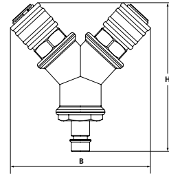
Distributor with 2 quick disconnect couplings with push-in plug
